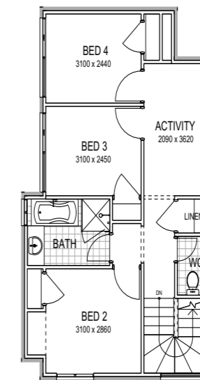
UPPER FLOOR PLAN 1:100
